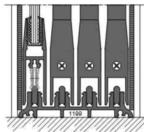
3 Rail Tracks
